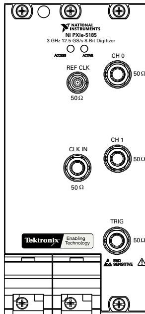
Figure 7. NI 5185 (50 \Omega )
